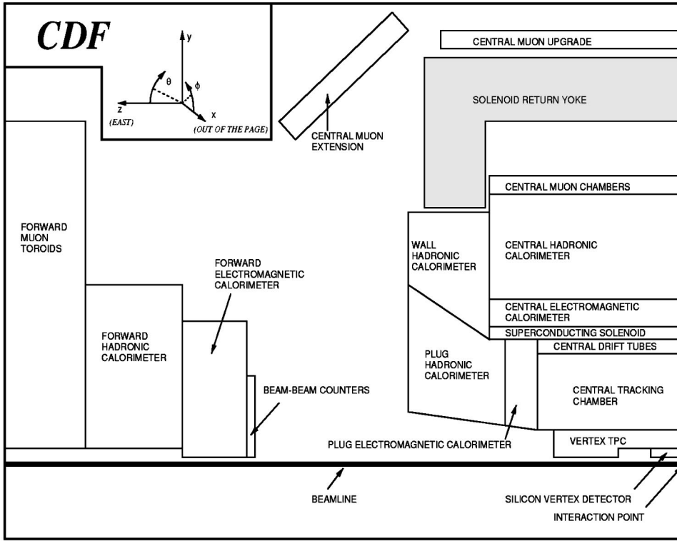
FIG. 1. Side view of one quadrant of the CDF detector for run 1. The detector is symmetric about the interaction point.
