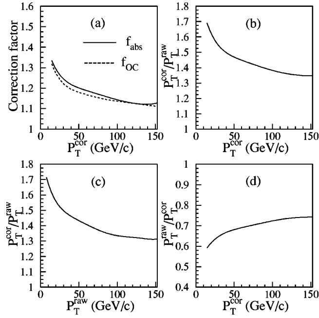
FIG. 4. “Flavor-independent” jet corrections, for a jet clustering cone of R=0.4 . (a) Absolute correction, f_{\text{abs}} , and out-of-cone correction factor, 1+OC/P_T , versus corrected jet P_T , P_T^{\text{cor}} . (b) Total correction, P_T^{\text{cor}}/P_T^{\text{raw}} , as a function of P_T^{\text{cor}} . (c) Total correction, P_T^{\text{cor}}/P_T^{\text{raw}} , as a function of P_T^{\text{raw}} . (d) Fraction of measured momentum, P_T^{\text{raw}}/P_T^{\text{cor}} versus P_T^{\text{cor}} .
